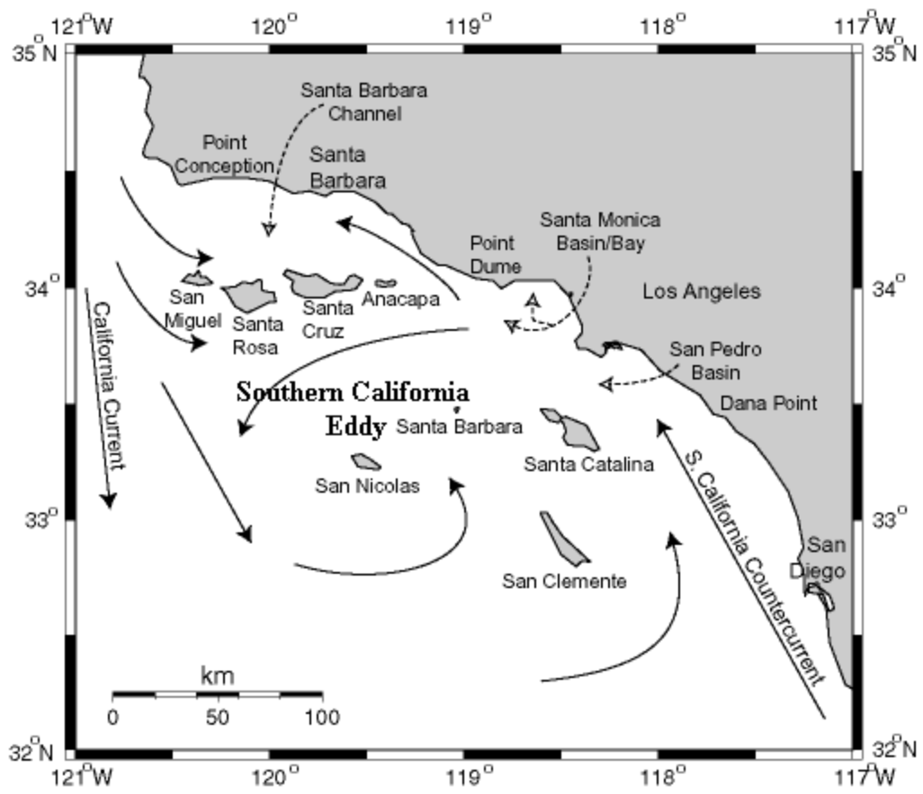
(After Hickey, B. M., 1992, Progress in Oceanography, V30: 37-115)
